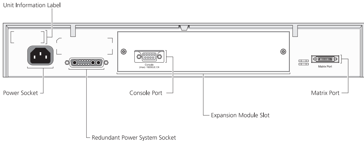
Figure 3 VCN Services Switch 100 - Rear View
